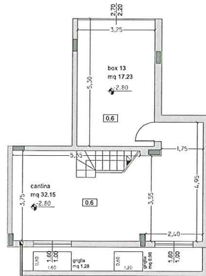
PIANO INTERRATO
